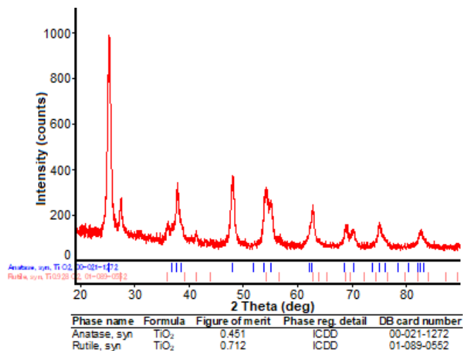
Fig 3. XRD diagram and the result of qualitative analysis of 1.1 %wt Cr-doped TiO 2
