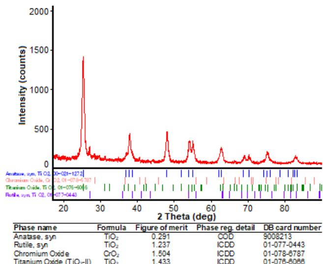
Fig 4. XRD diagram and the result of qualitative analysis of 3.9 %wt Cr-doped TiO 2
