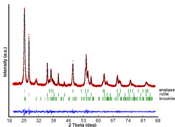
Fig 7. X-ray diffraction Fullprof Patern Matching of undoped TiO 2
