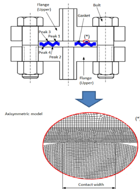
Fig. 1 Schematic of gasket tightening by the flange
