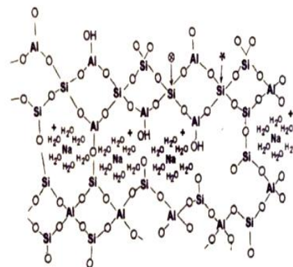
Fig.1. Proposed structure of a Na-polysialate polymer
