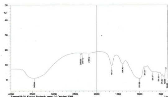
Fig 5b. Infrared Spectra of Na-Geopolymer-Cr (20ppm Cr)
