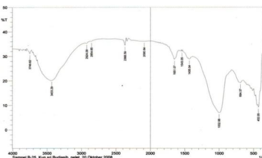
Fig 5c. Infrared Spectra of Na-Geopolymer-Cr (25ppm Cr).
