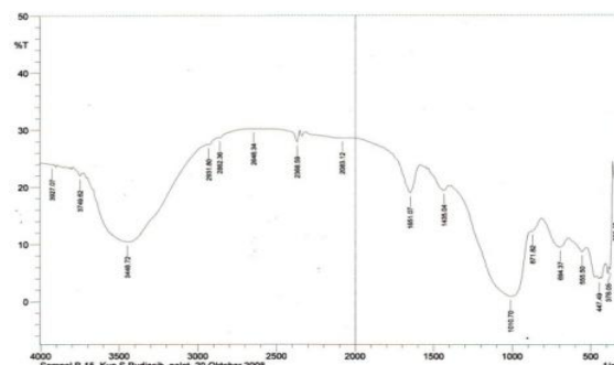
Fig 5.a. Infrared Spectra of of Na-Geopolymer-Cr (15ppm Cr)
