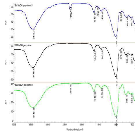
Fig.4. Infrared spectra of Na-Geopolymer made by 8,10,12 M NaOH.
