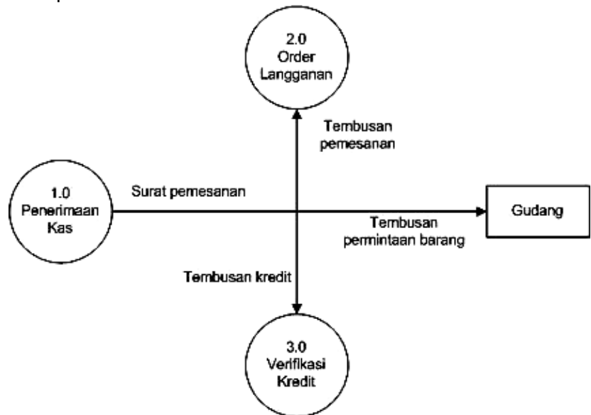
Gambar 11. Diverging DFD
