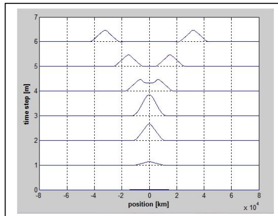
Gambar 4. Elevasi di permukaan saat t = 1s, t = 3s, t = 7s, t = 10s, t = 25s, t = 50s and t = 100s .
